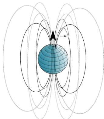
Figure 2- Magnetic field lines Source: Creative Commons CC0 https://pixabay.com/photo-154887/
